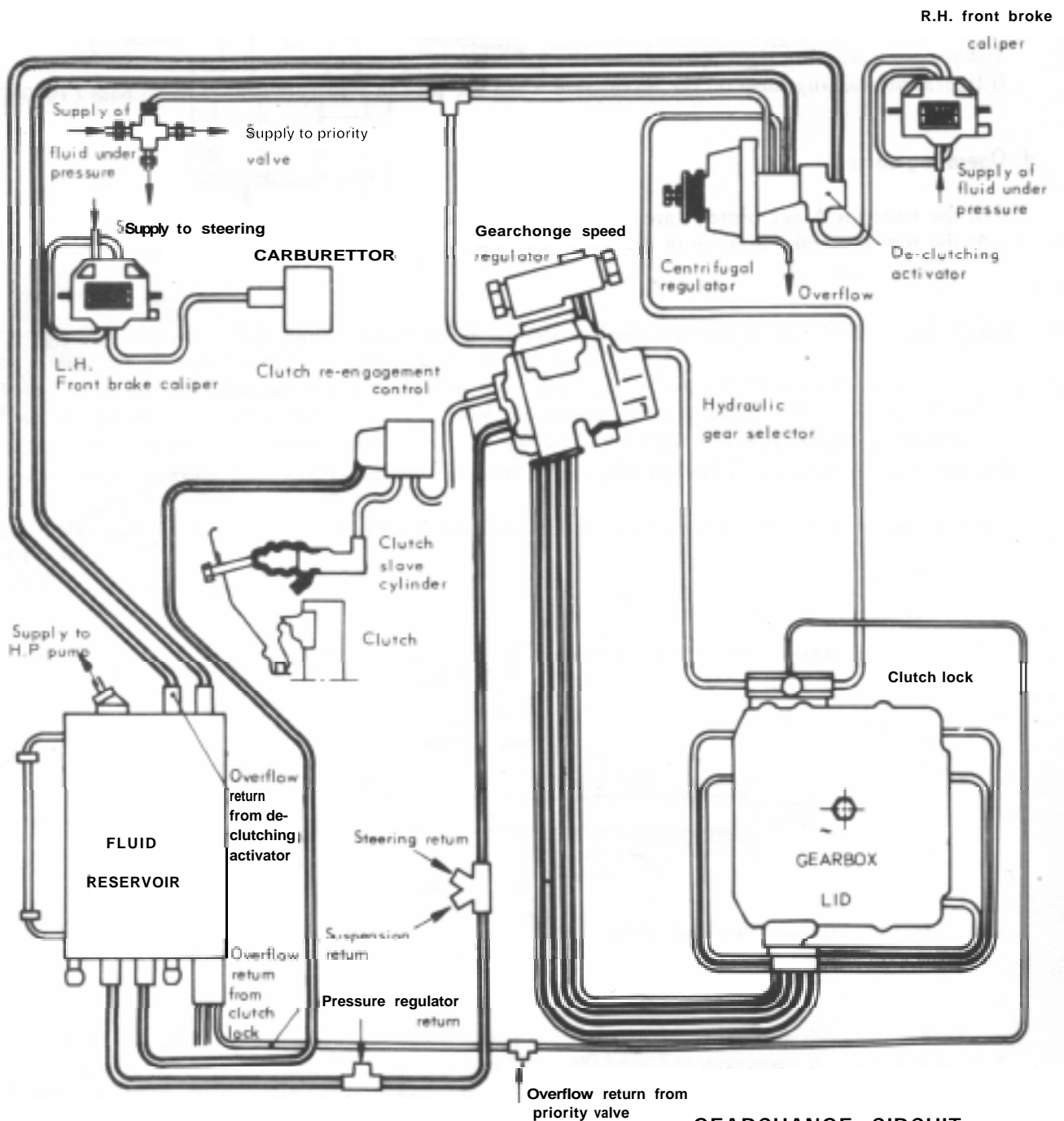
GEARCHANGE CIRCUIT
